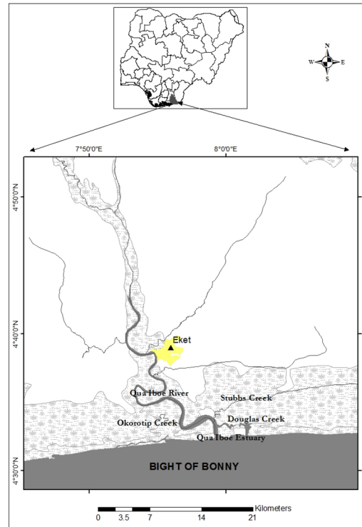
Fig 1. Map of study area showing the ecosystems in Niger Delta region of Nigeria (Inset: Map of Nigeria).
